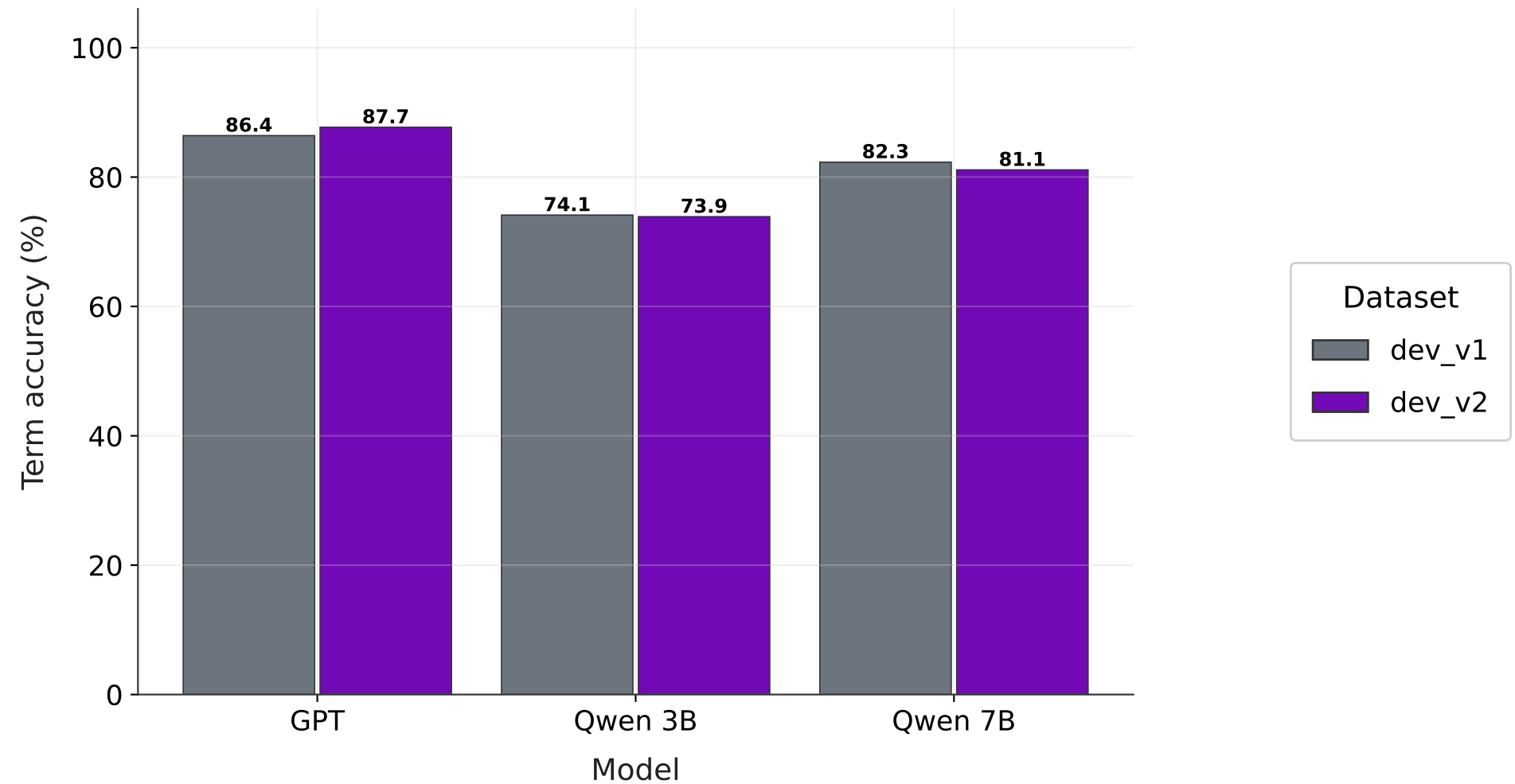
dev_v1 vs. dev_v2 (random_term; macro avg over language pairs; per model)
