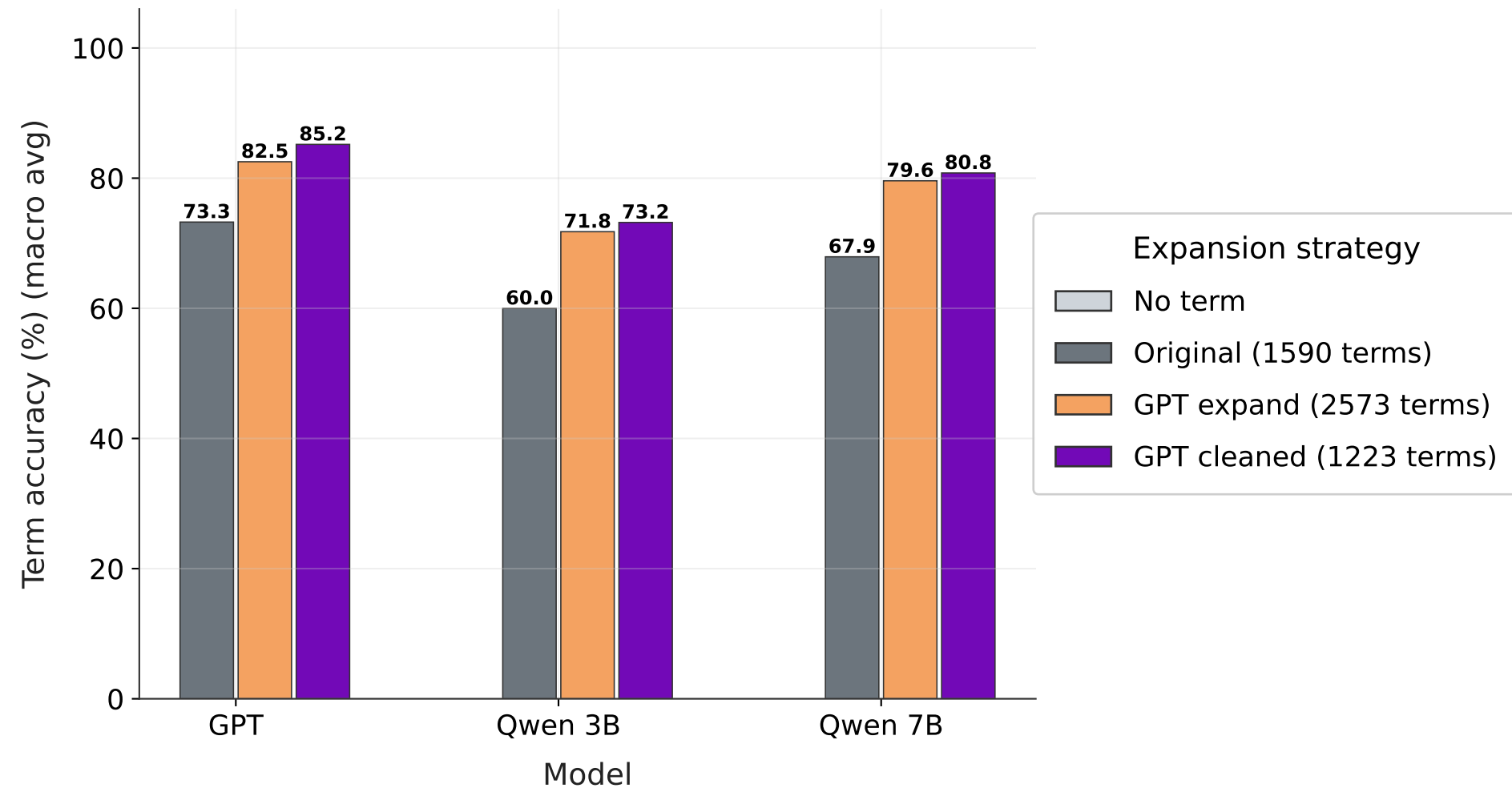
Proper Terms Expansion: Original vs GPT Expand vs GPT cleaned (GPT-4o-mini, Qwen2.5-3B, Qwen2.5-7B; proper_term)
