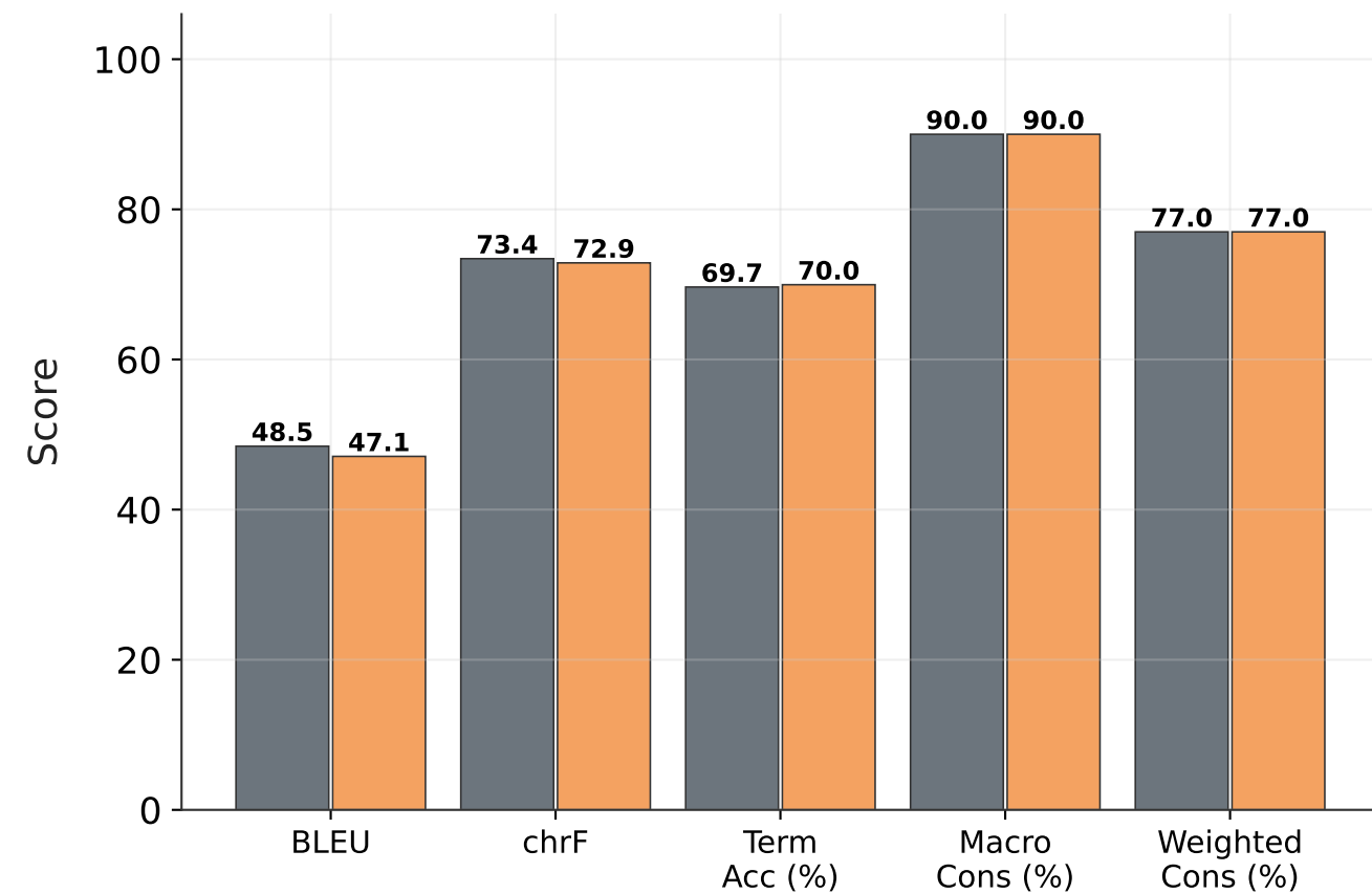
Qwen 7B — LoRA (1 epoch)
