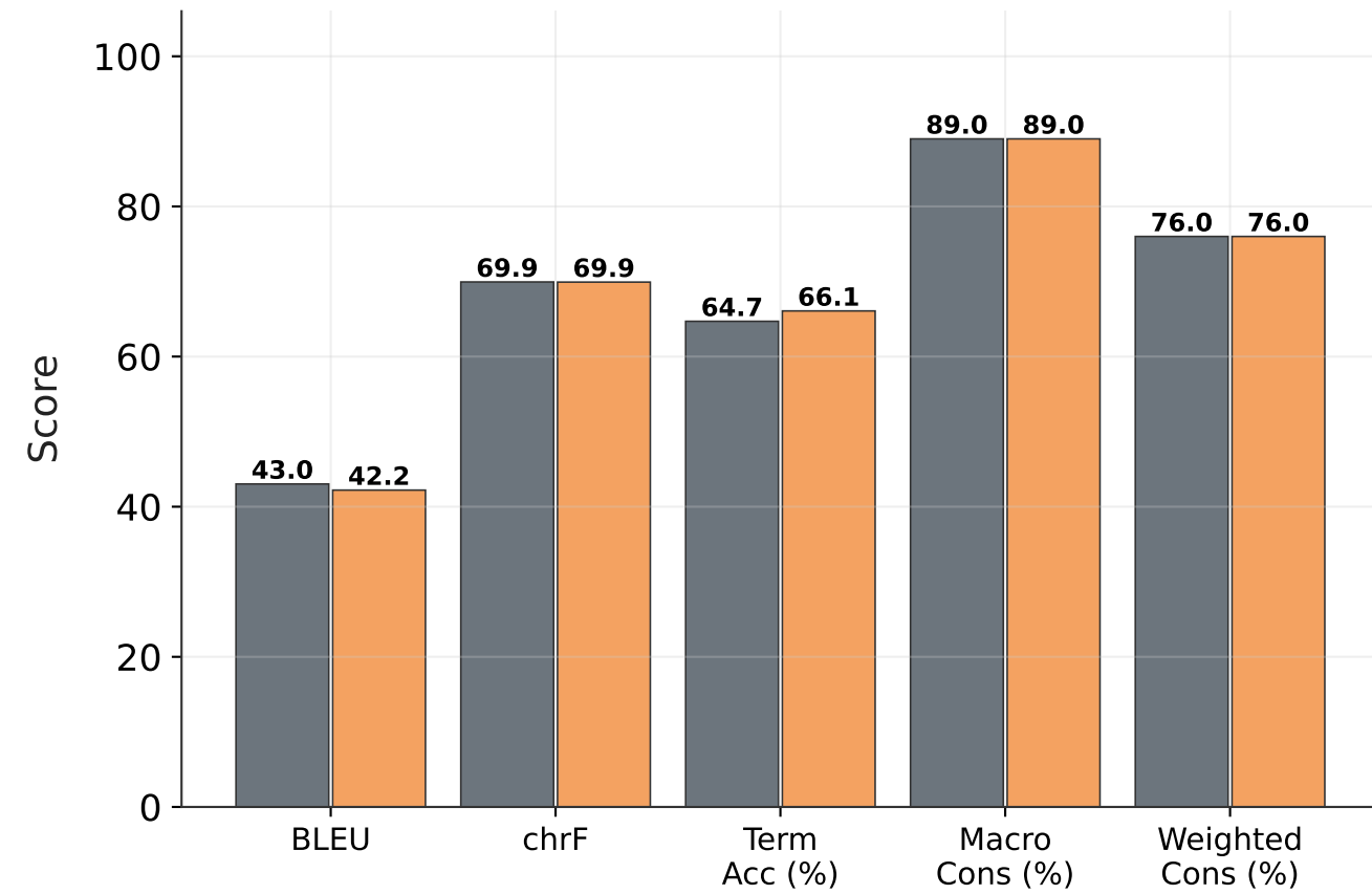
Qwen 3B — LoRA (1 epoch)
