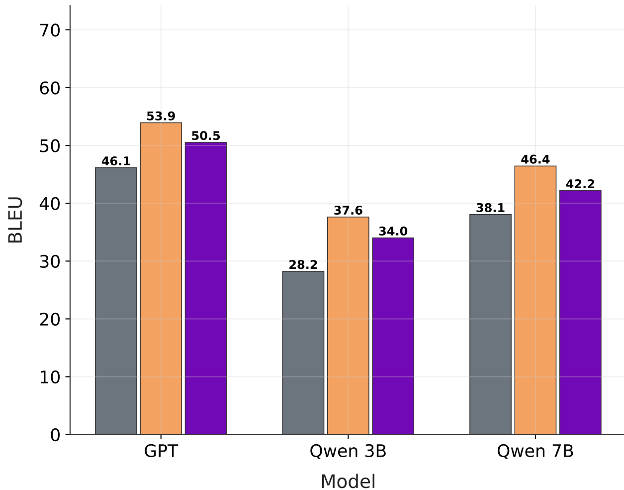
Proper Terms Expansion: Original vs GPT Expand vs GPT cleaned (GPT-4o-mini, Qwen2.5-3B, Qwen2.5-7B; proper_term; macro avg over language pairs)
