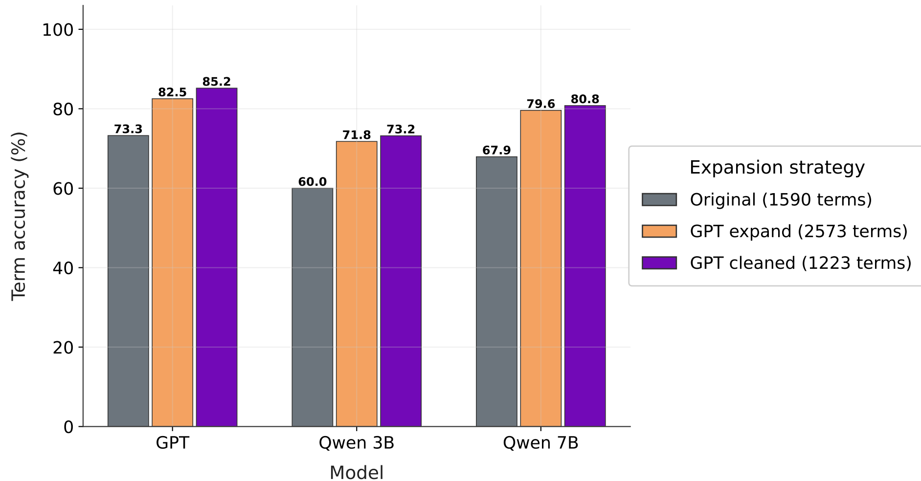
Proper Terms Expansion: Original vs GPT Expand vs GPT cleaned (GPT-4o-mini, Qwen2.5-3B, Qwen2.5-7B; proper_term; macro avg over language pairs)
