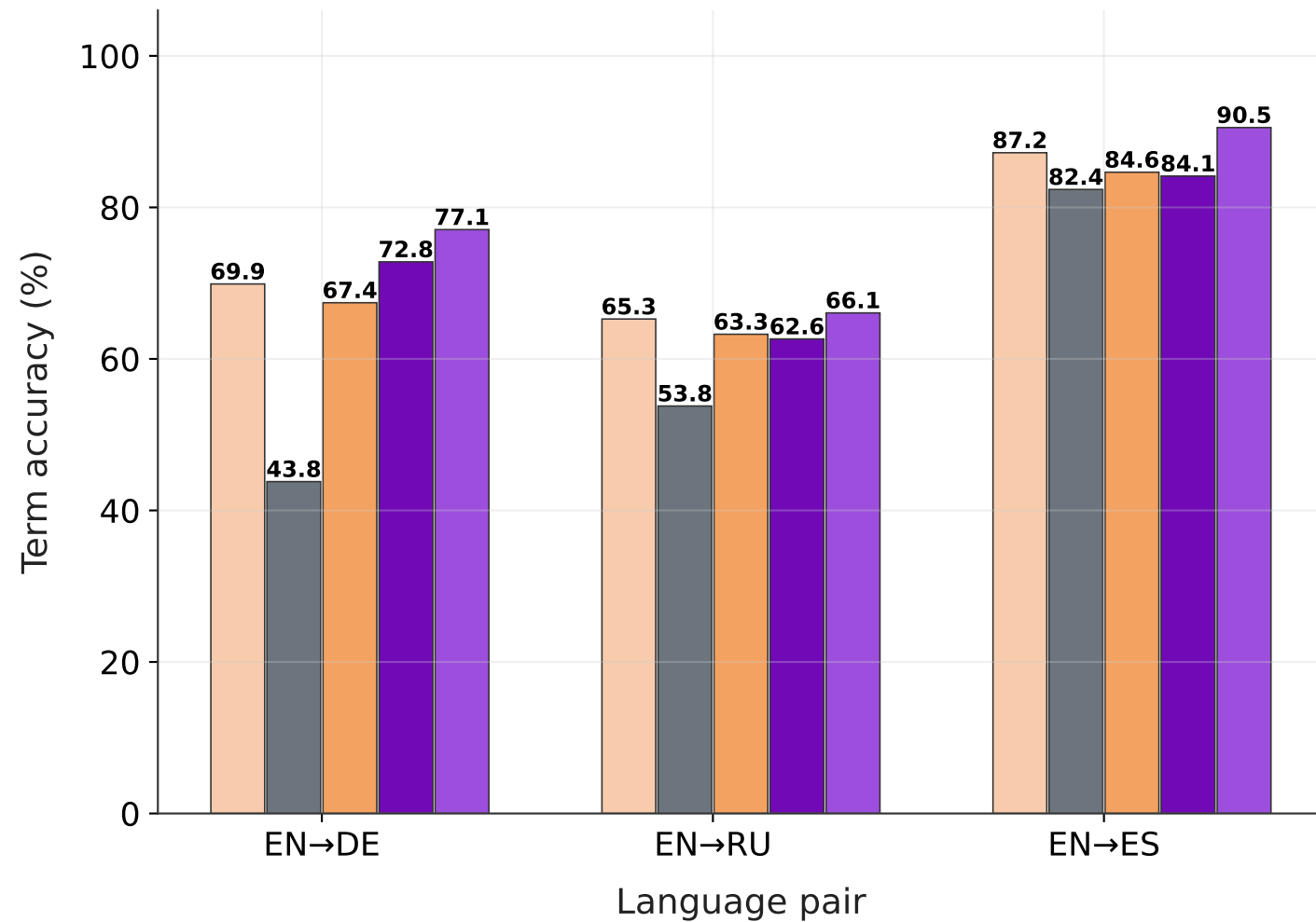
Terminology expansion by language pair (dev_v1; Qwen 3B)
