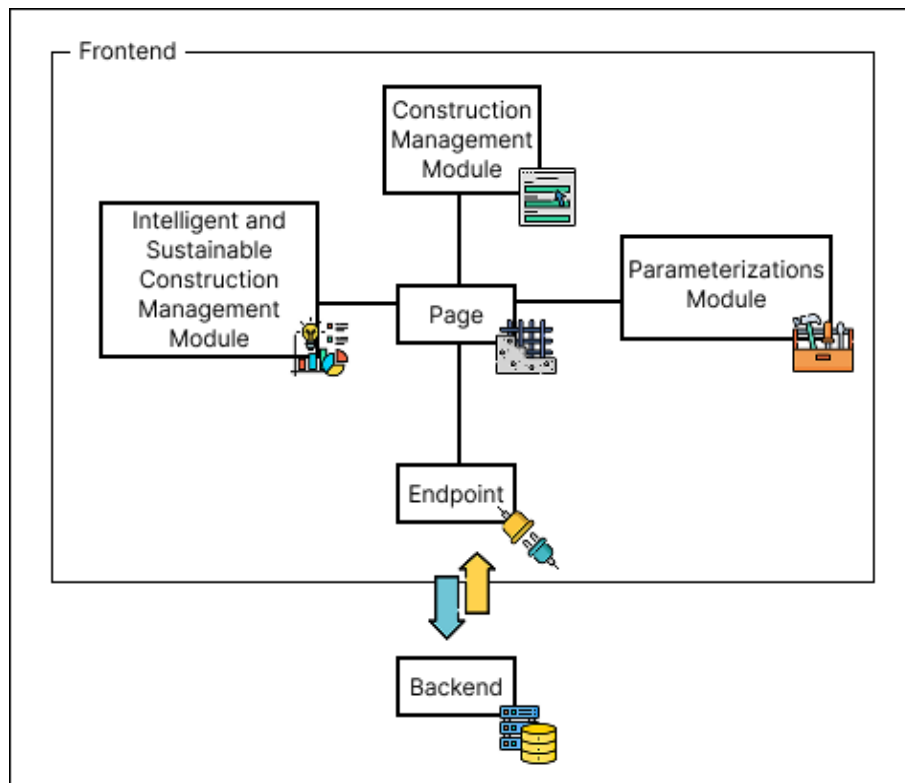
Figure 12: Logical solution architecture
