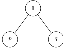
Figura 14.1: Diagrama representando o forcing poset \mathbb{P} = \{\mathbb{1}, p, q\} .
