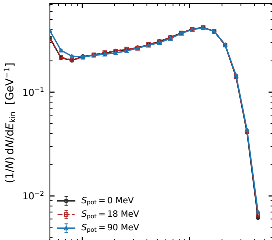
primary neutrons, HGND front-face acceptance
