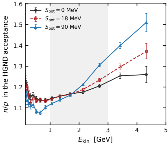
nucleon ratio against energy
