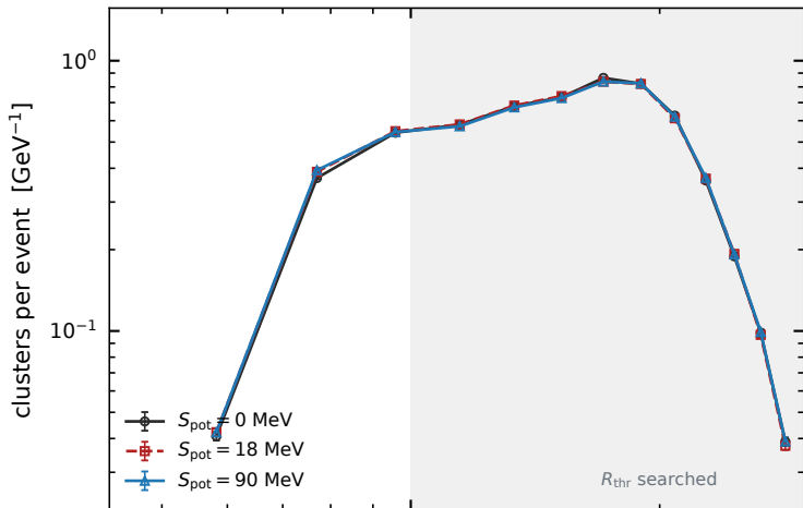
reconstructed neutron candidates, purity-locked selection
