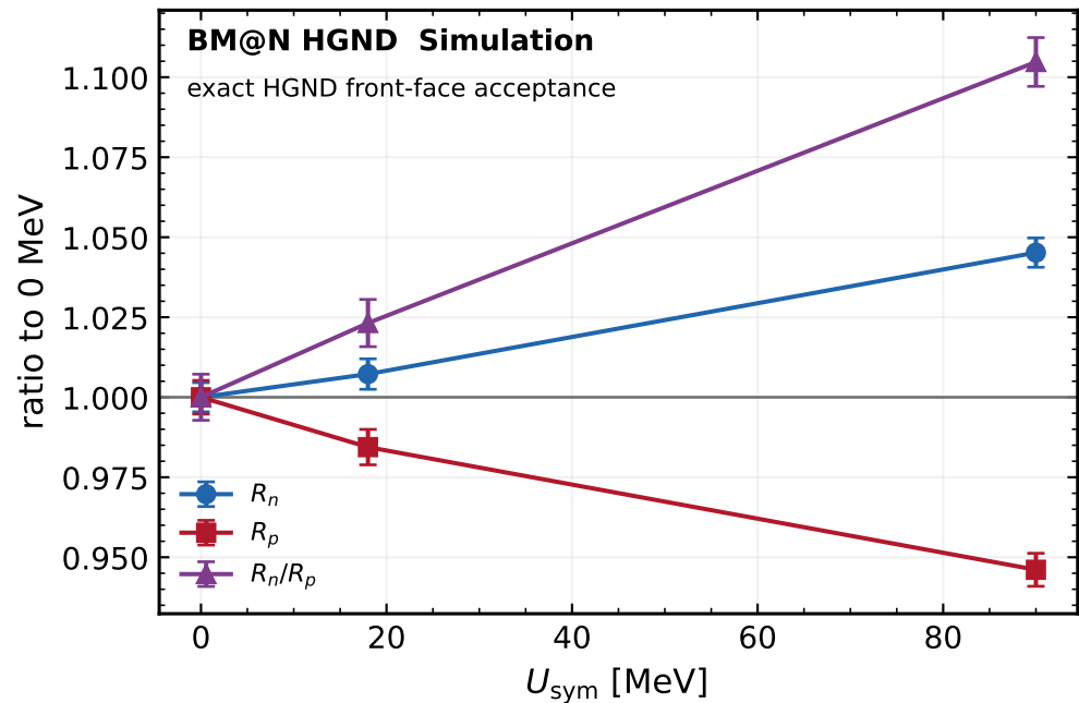
Spectral shape: monotonic isovector response
