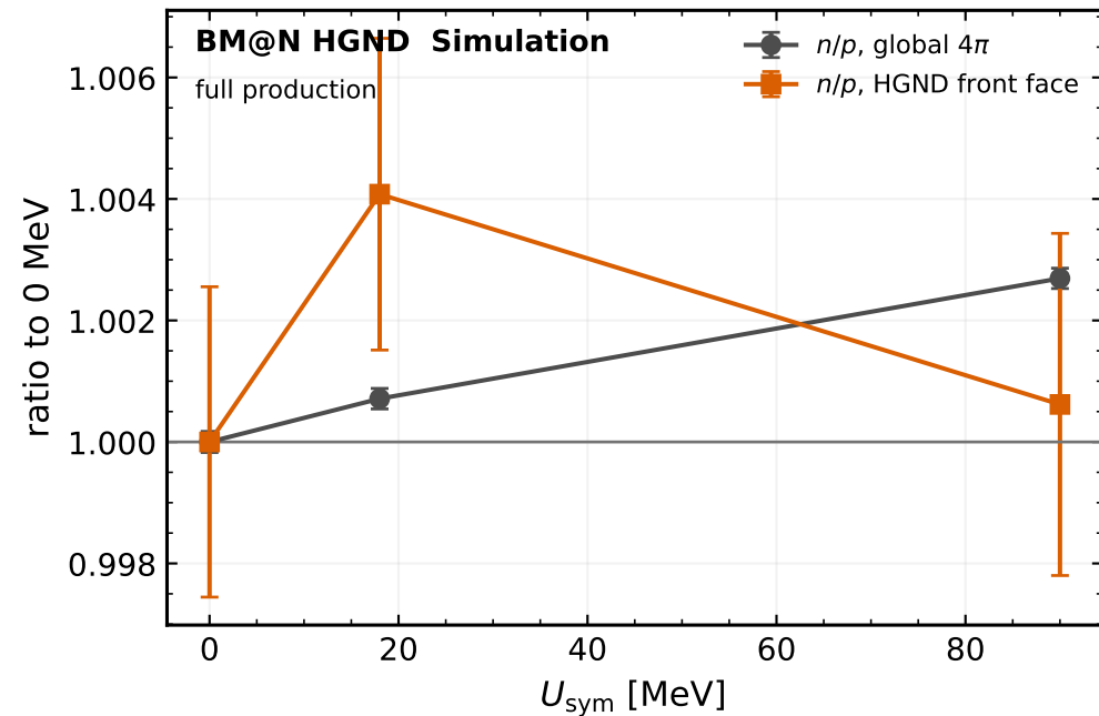
Yield ratio: small or null response
