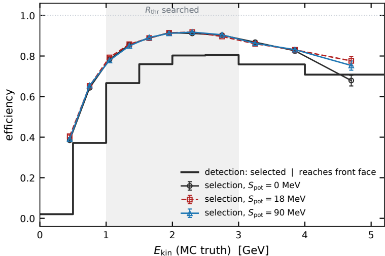
Neutron efficiency against true energy (MC truth)
