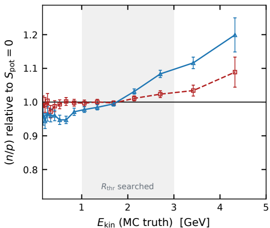
the isovector signal, against energy (MC truth)
