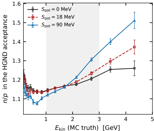
nucleon ratio against energy (MC truth)
