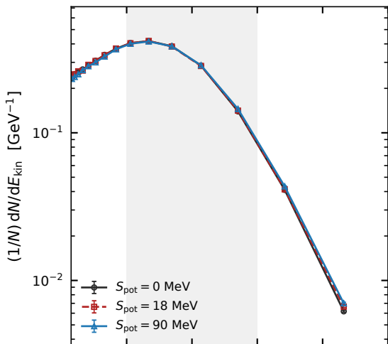
primary neutrons, HGND front-face acceptance (MC truth)
