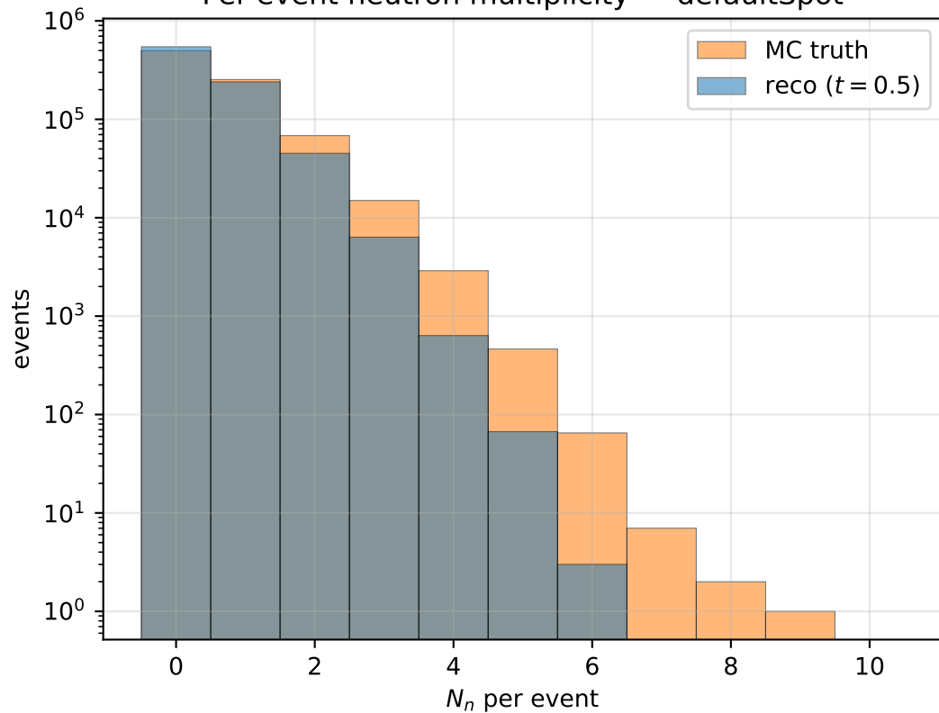
Per-event neutron multiplicity — defaultSpot
