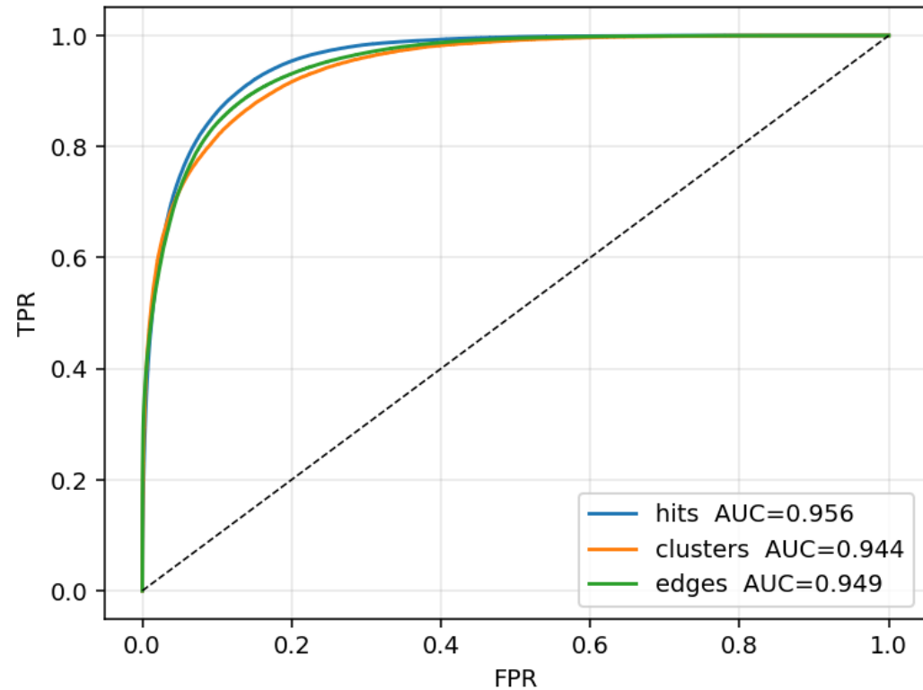
ROC — HPC checkpoint on defaultSpot test split
