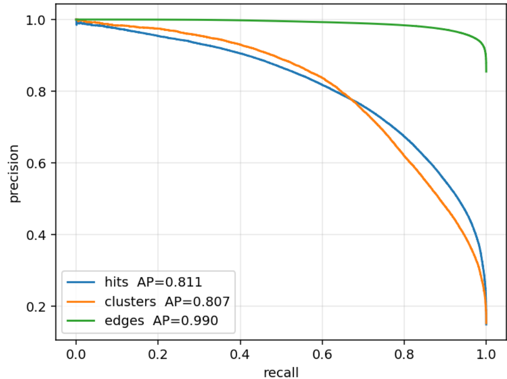
Precision-recall
