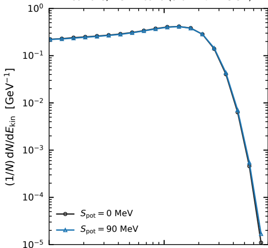
neutrons, HGND band ( 9.0^\circ < \theta < 13.5^\circ )
