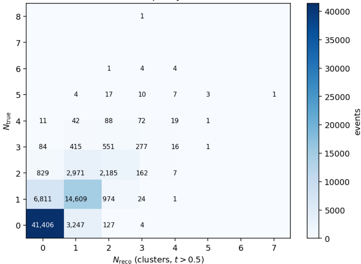
Neutron-multiplicity confusion
