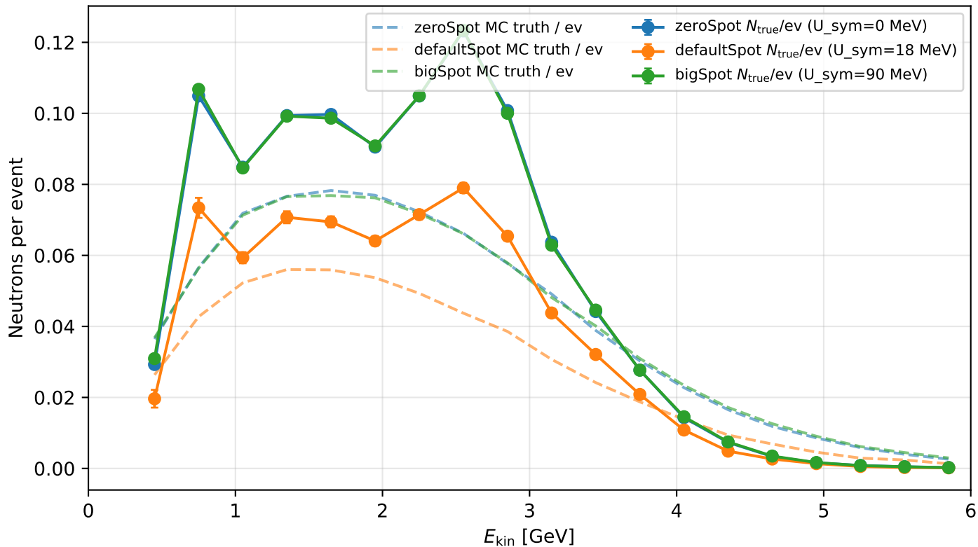
Efficiency-corrected yield N_{\text{true}} vs. MC truth ( t = 0.5 )
