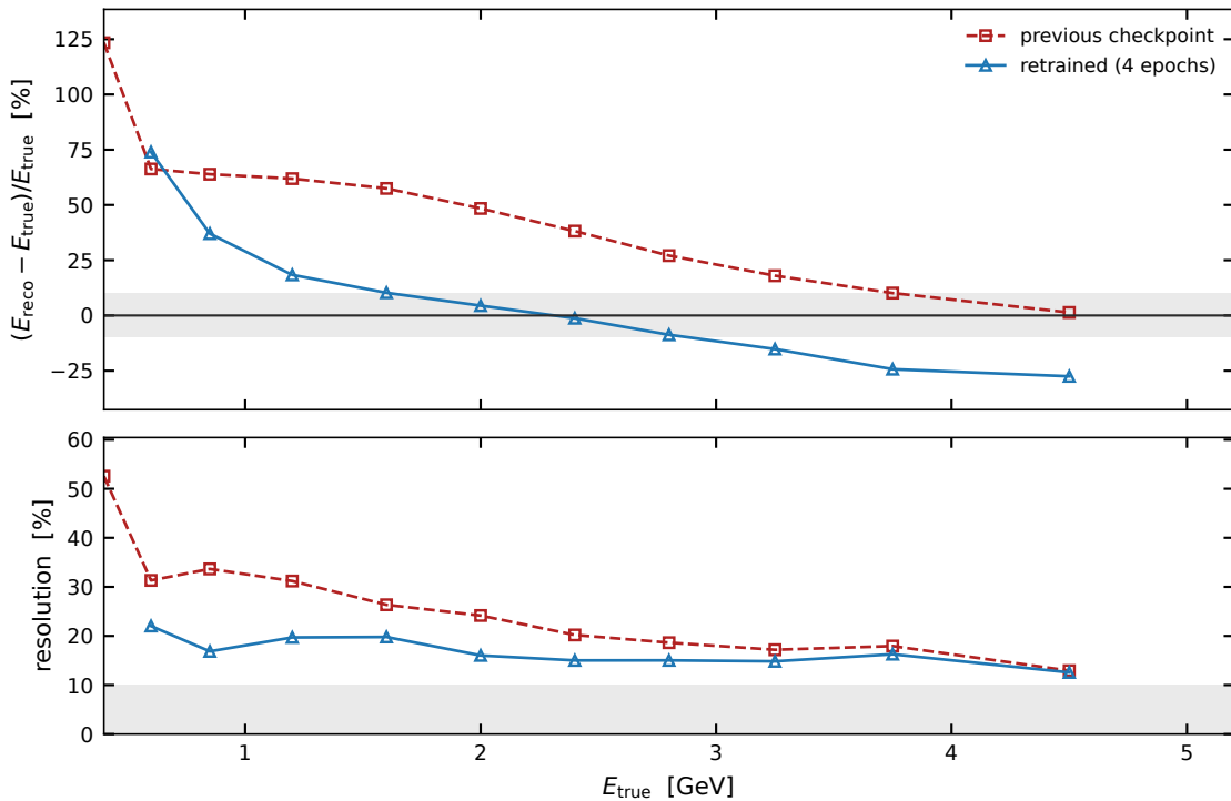
Energy linearity and resolution against the reference targets (shaded: 10 %)
