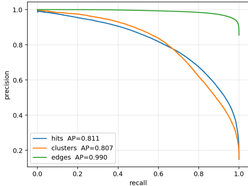
Precision-recall
