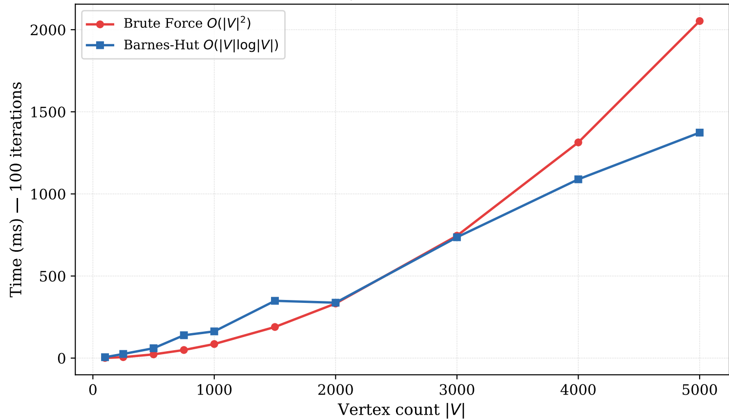
Force-Directed Layout — Runtime vs Graph Size
