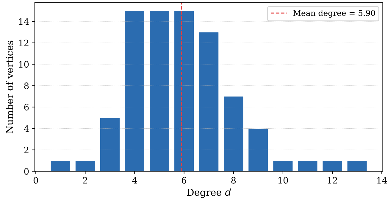
Erdős-Rényi Graph — Degree Distribution
