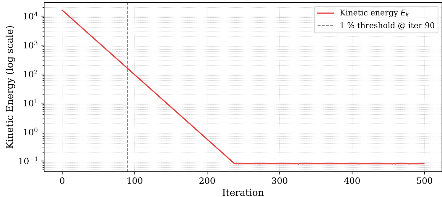
Fruchterman-Reingold — Convergence Curve
