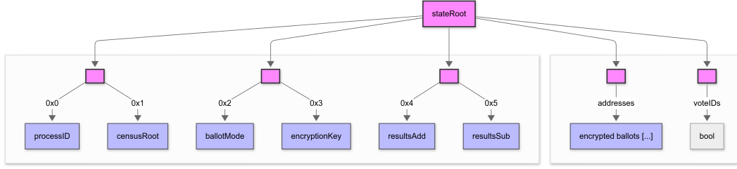
Fig. 2. Structure of the state Merkle tree. The first leaves are reserved for global process parameters while subsequent leaves store encrypted ballots indexed by voter addresses and vote identifiers.
