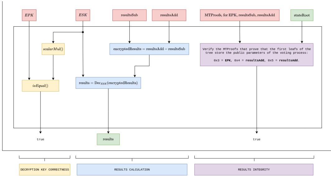
Fig. 7. Results circuit. All public values are framed in green.
