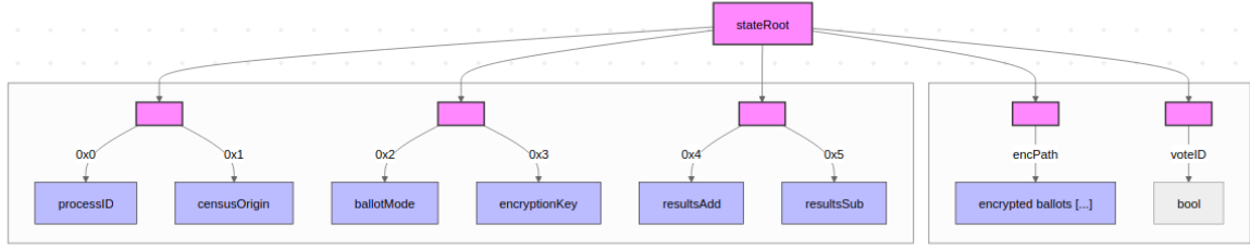
Fig. 1: Structure of the state Merkle tree. The first leaves are reserved for global election parameters while subsequent leaves store vote identifiers and encrypted ballots.
