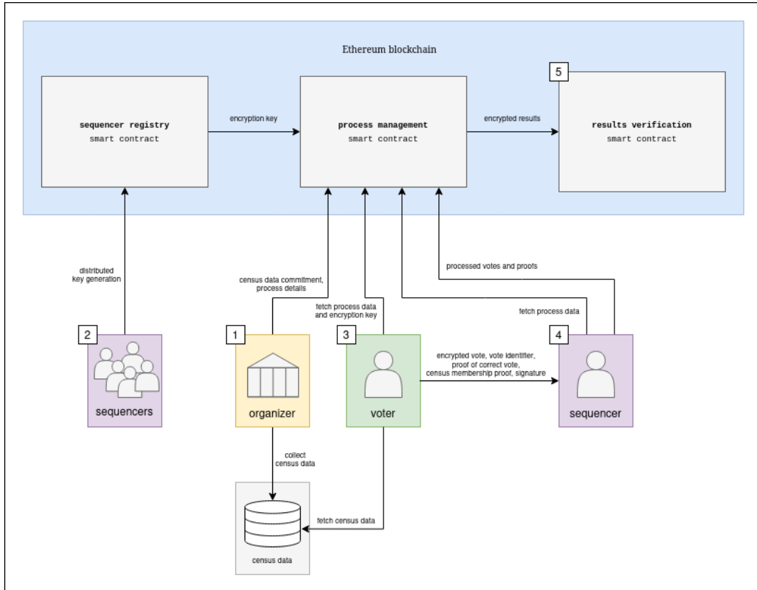
Fig. 1. Overview of the protocol flow.
