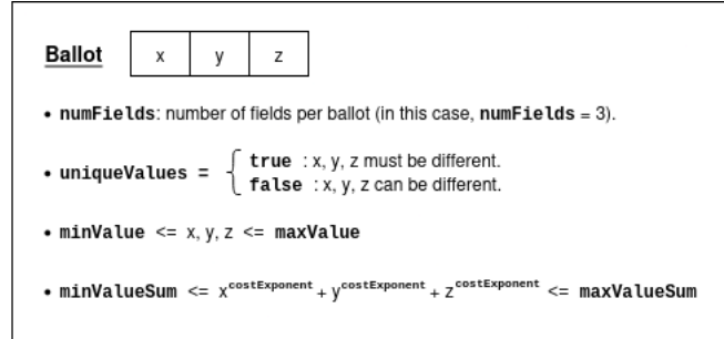
Fig. 9. Schematic representation of the parameters that define a ballot in DAVINCI.
