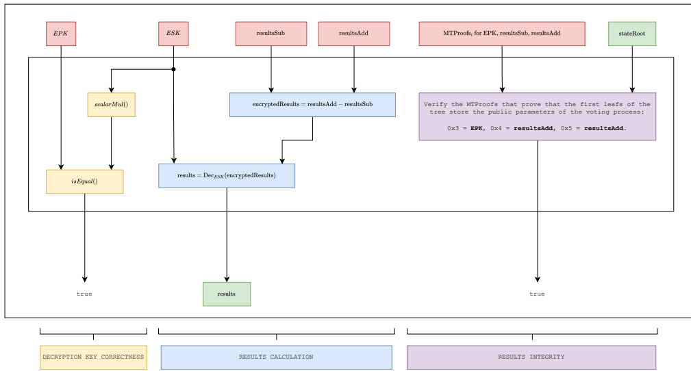
Fig. 7. Results circuit. All public values are framed in green. The figure is not right.
