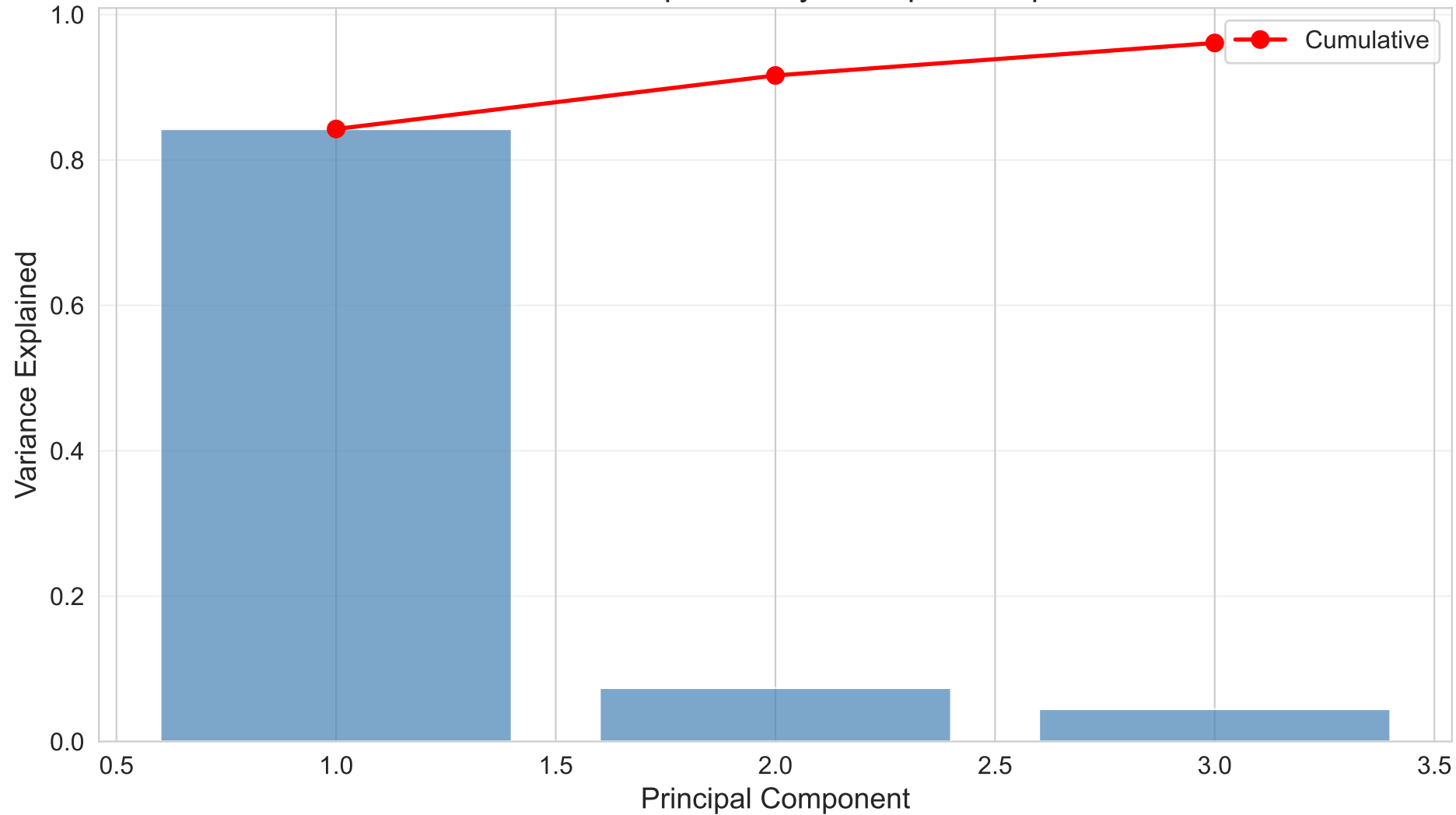
PCA: Variance Explained by Principal Components
