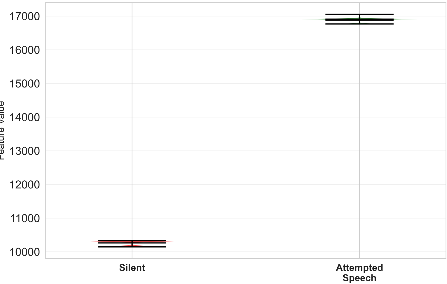
Feature 10 Correlation: 0.649
