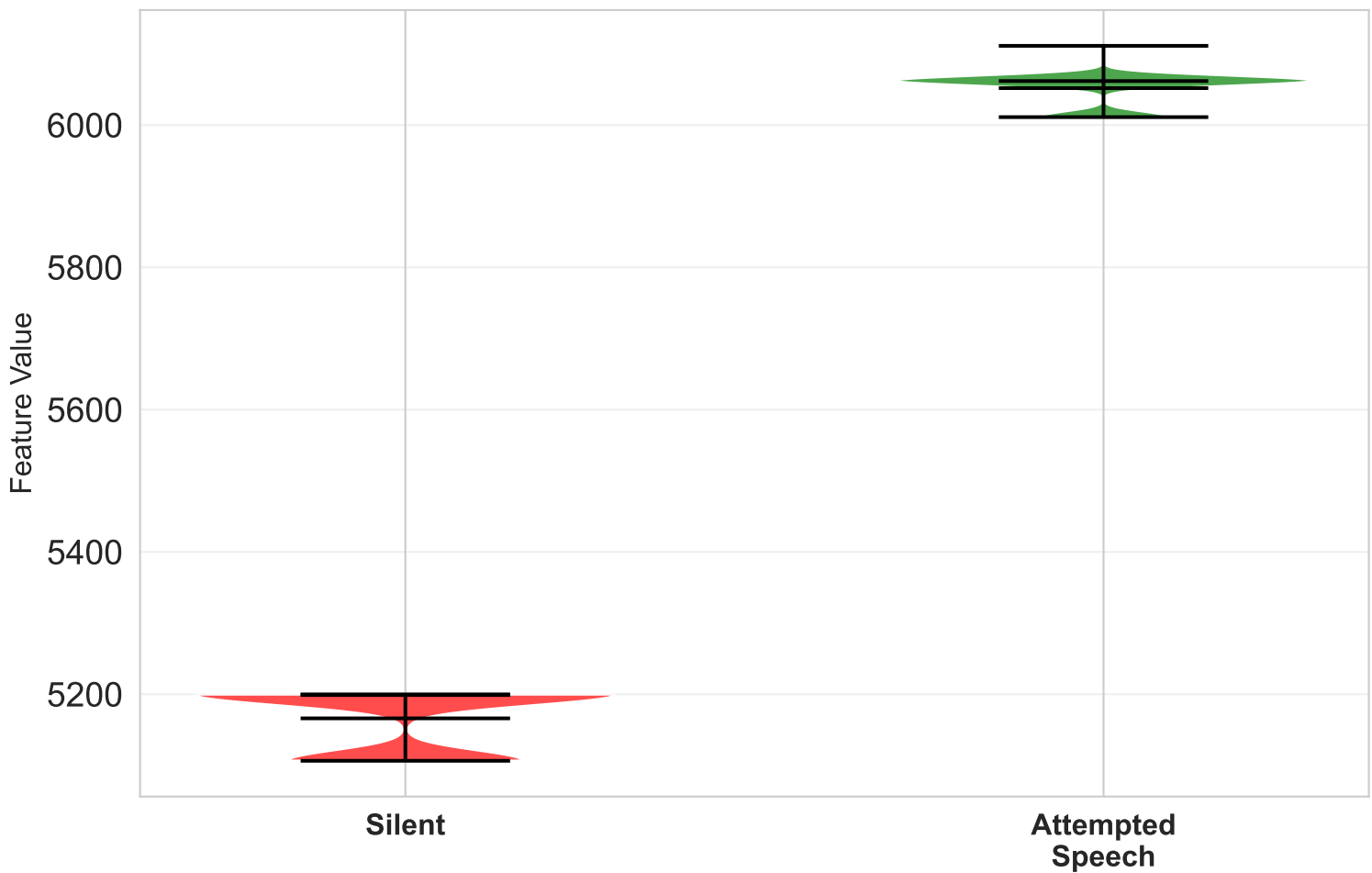
Feature 0 Correlation: 0.641
