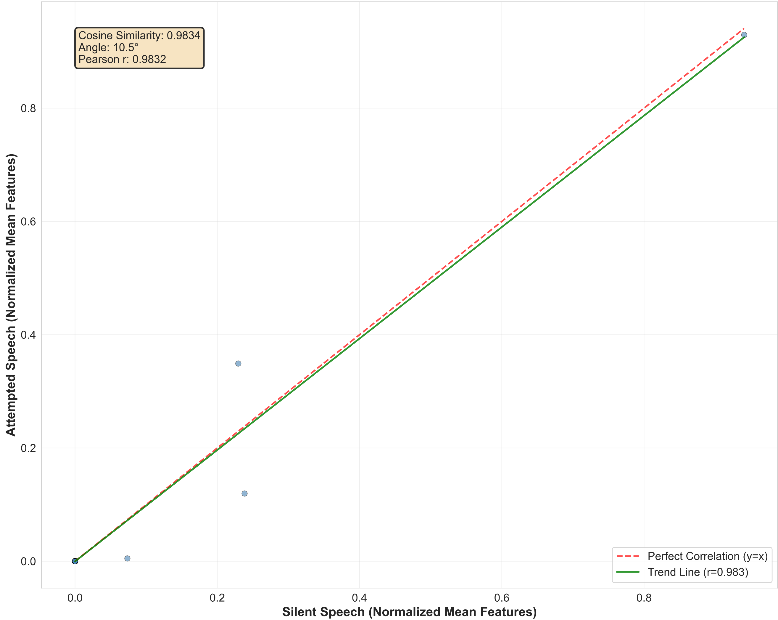
Feature Space Correlation: Silent vs Attempted Speech Cosine Similarity: 0.9834 (98.34%) | Pearson r: 0.9832 | Angle: 10.5°
