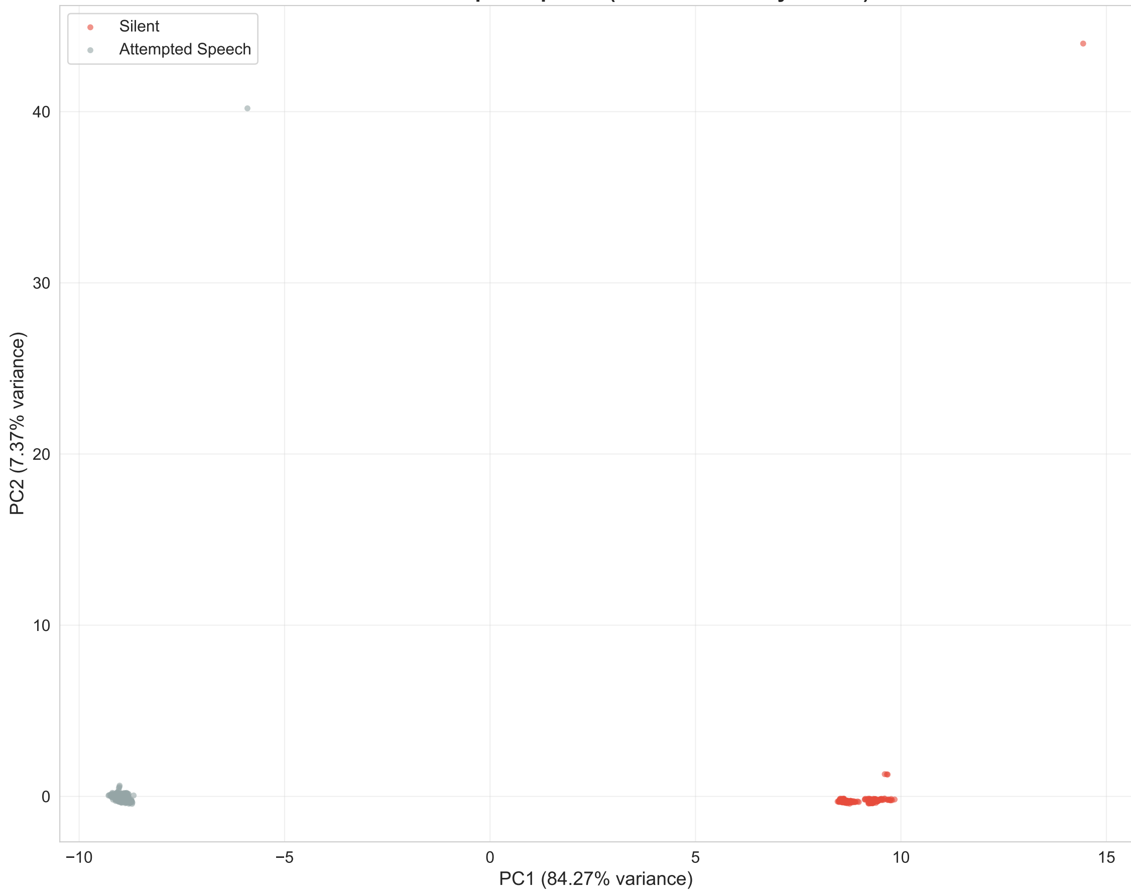
PCA: Feature Space Overlap Silent vs Attempted Speech (Cosine Similarity: 98.3%)
