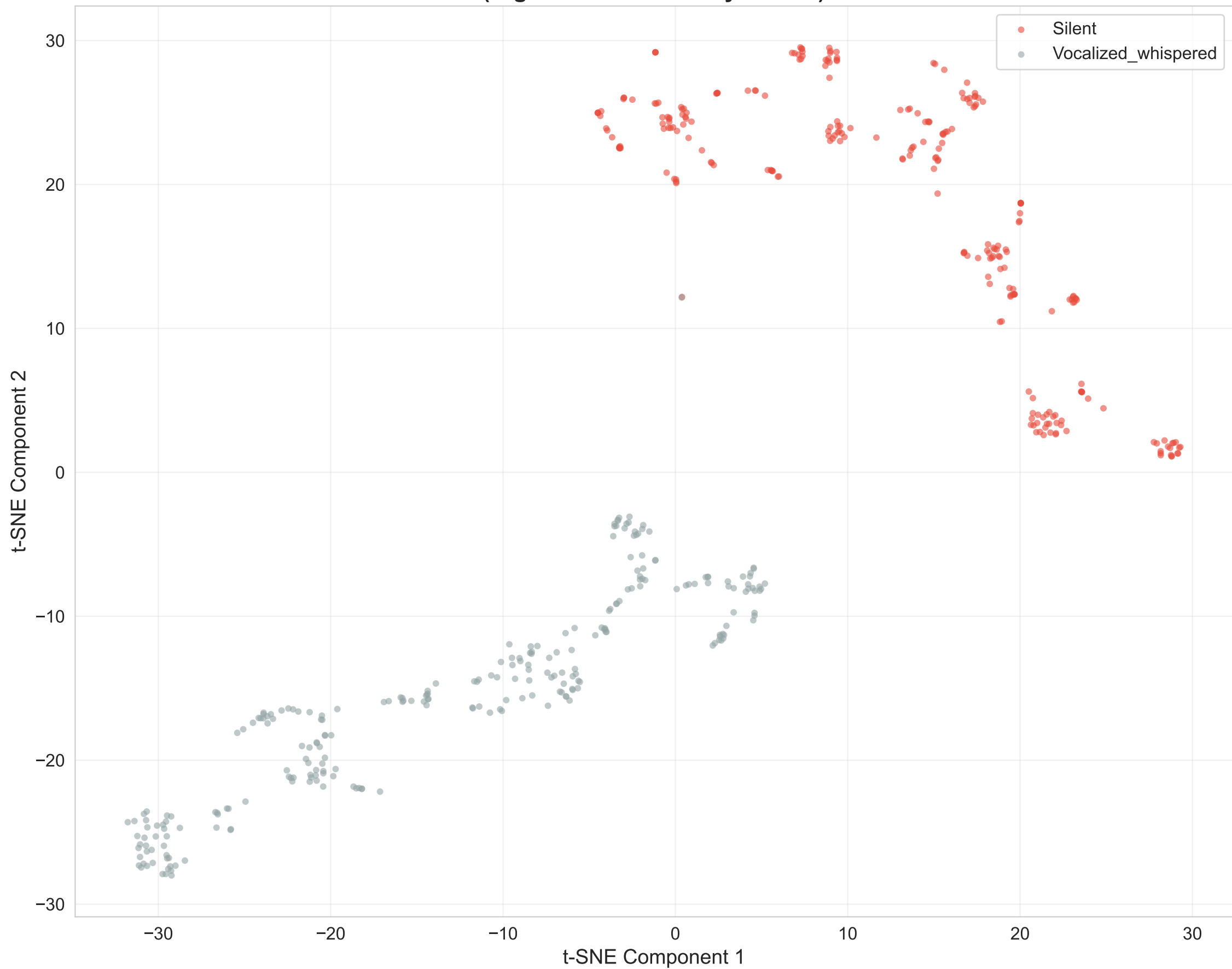
EMG Feature Space: Silent vs Attempted Speech (High Cosine Similarity: 98.3%)
