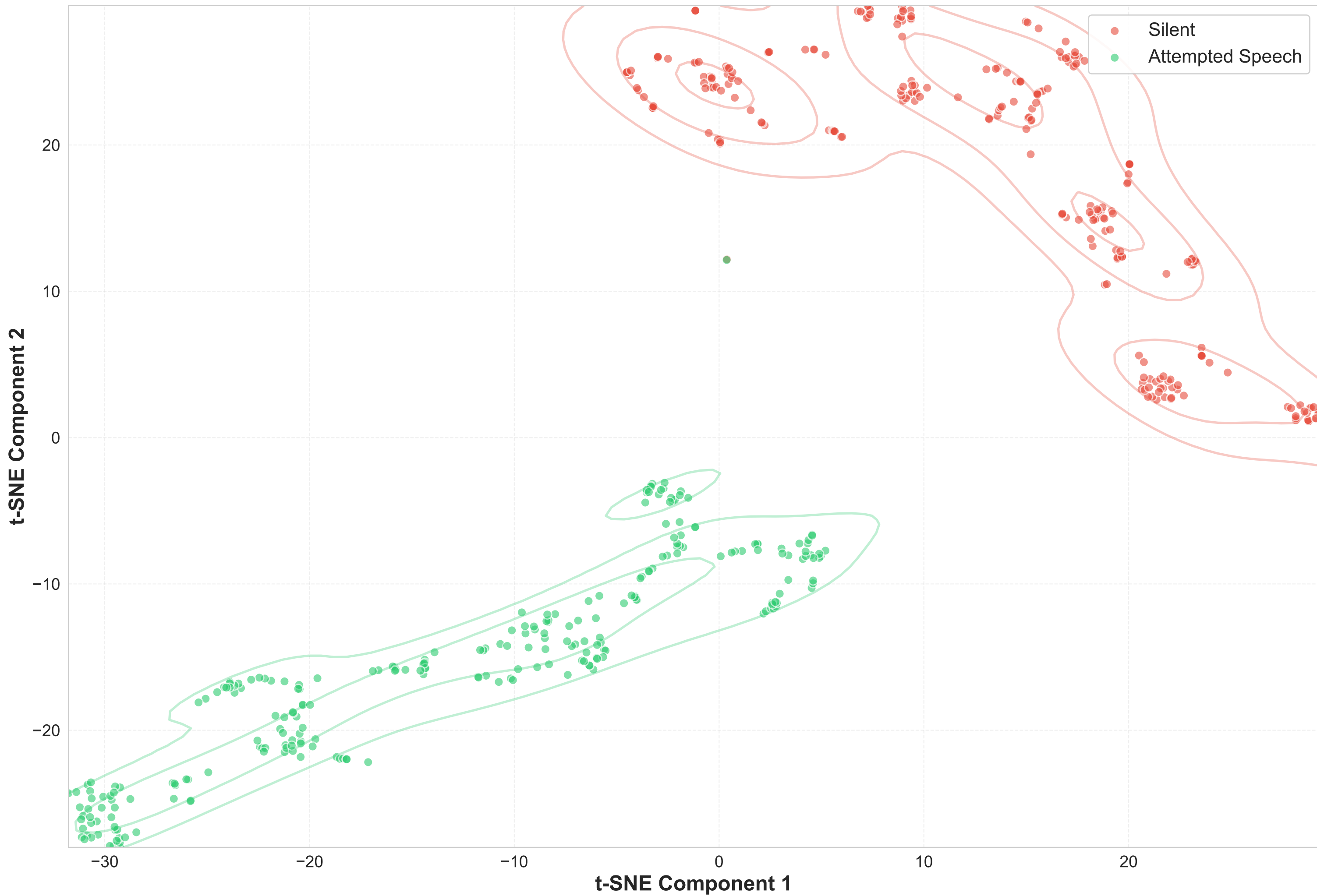
Feature Space Overlap: Silent vs Attempted Speech Cosine Similarity: 0.9834 (98.34%) | Angle: 10.5° (Contours show density of samples)
