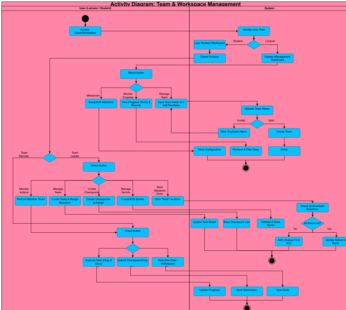
Activity Diagram: Team & Workspace Management
