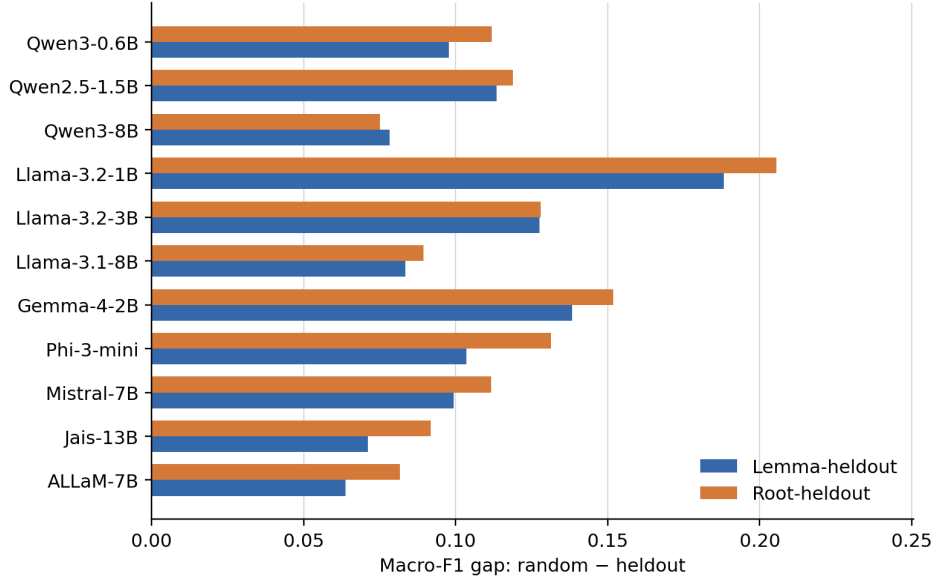
Fig. 1 Mean random-minus-heldout macro-F1 gaps for the eleven models, averaged over the three tasks and four representation interfaces. The two bars show lemma-heldout and root-heldout gaps. Model-level means are listed in Table 2; the complete model-by-task-by-interface values are available in the archived CSV artifact.
