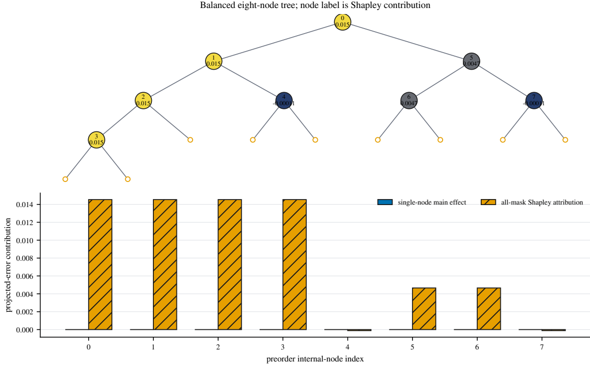
FIGURE 13. Attribution of the projected root error to individual vertices, for one balanced tree with eight internal vertices. All 2^8 = 256 subsets of vertices at which the closure residual is switched on were evaluated exhaustively; no sampling is involved. Vertex labels give the Shapley value of the resulting set function, and the lower panel compares single-vertex main effects with the full Shapley values. The efficiency residual is below 10^{-12} . The attribution is exact for this construction and is not a claim about a unique causal mechanism.
