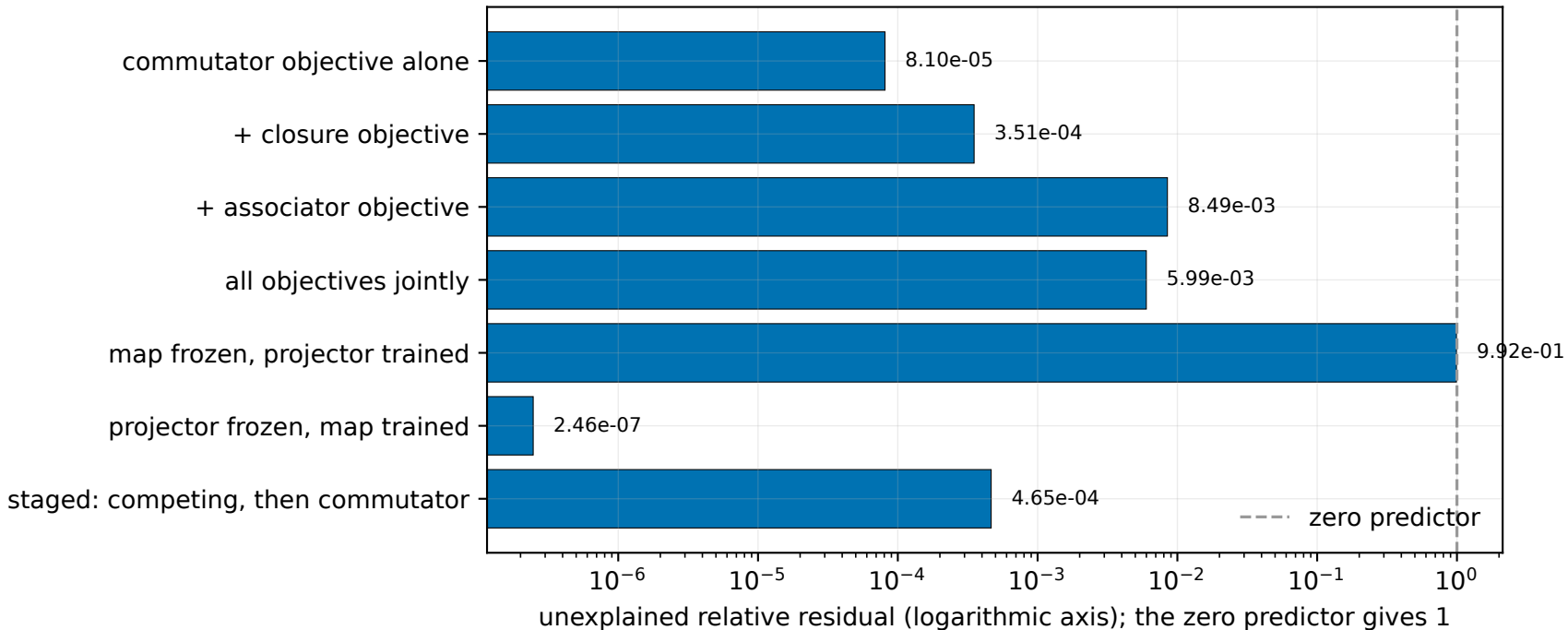
Ablation study of the commutator approximation
