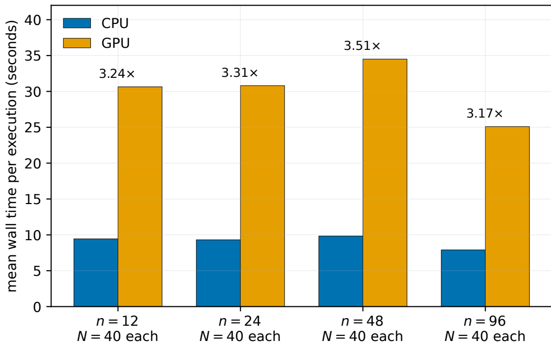
Mean wall time per execution, by device and ambient dimension (one machine; ratios annotated)
