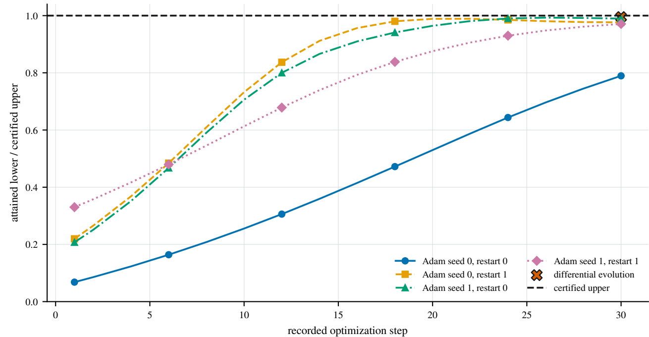
Every pilot trajectory; no failed search is hidden
