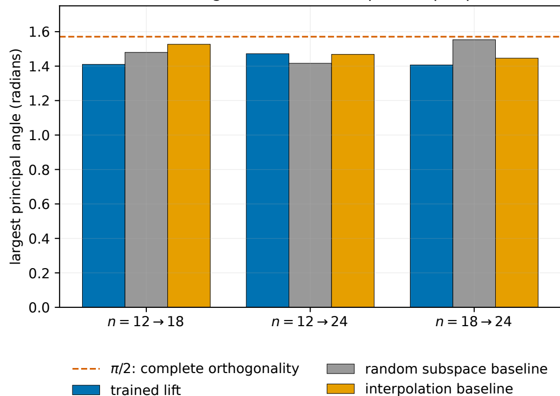
Transport of learned subspaces across three resolutions (one training run and one lift operator per pair)
