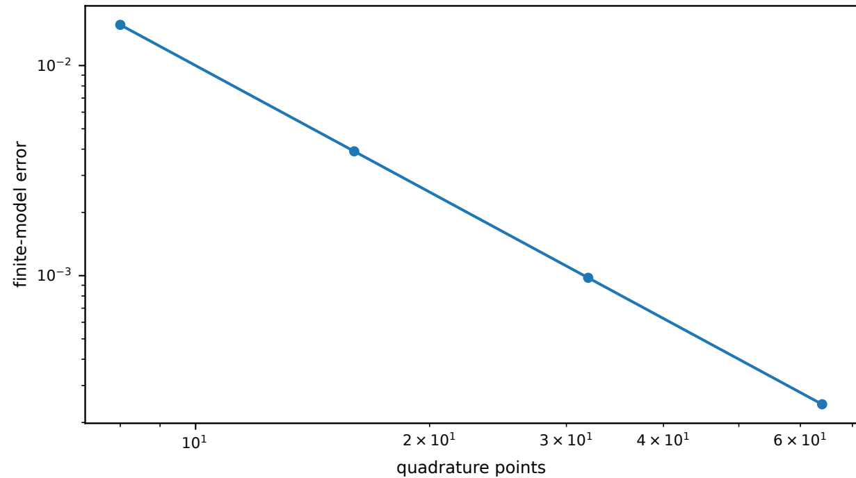
Quadrature Convergence
