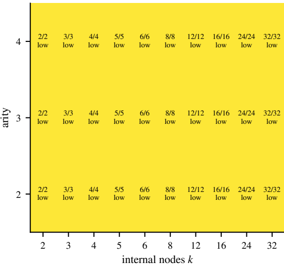
ambient; low strahler
