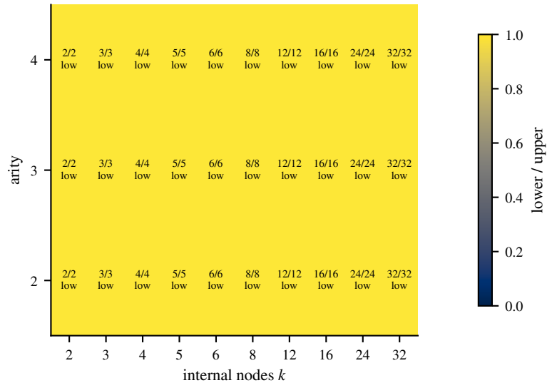
normal; low strahler
