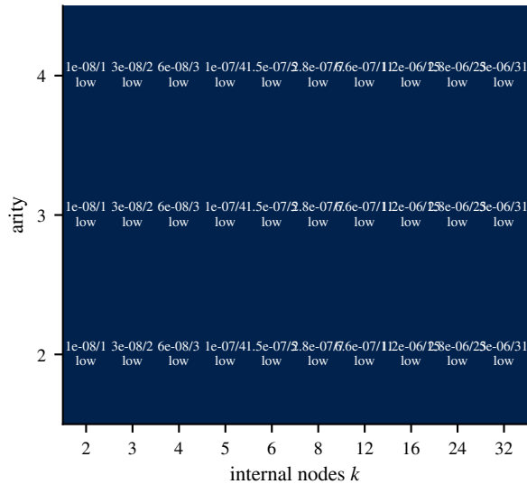
projected; low strahler
