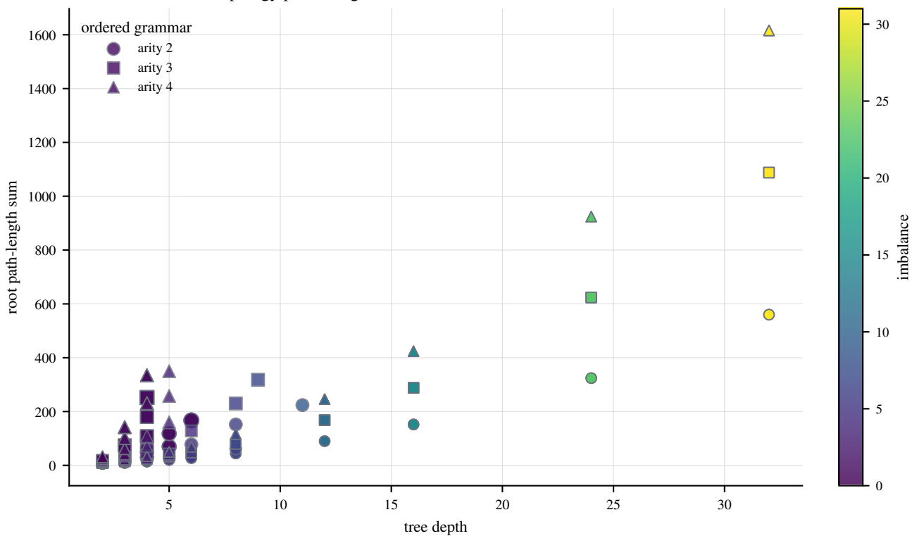
Topology phase diagram; marker size encodes Strahler number
