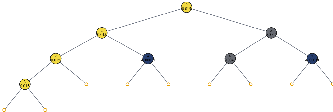
Balanced eight-node tree; node label is Shapley contribution
