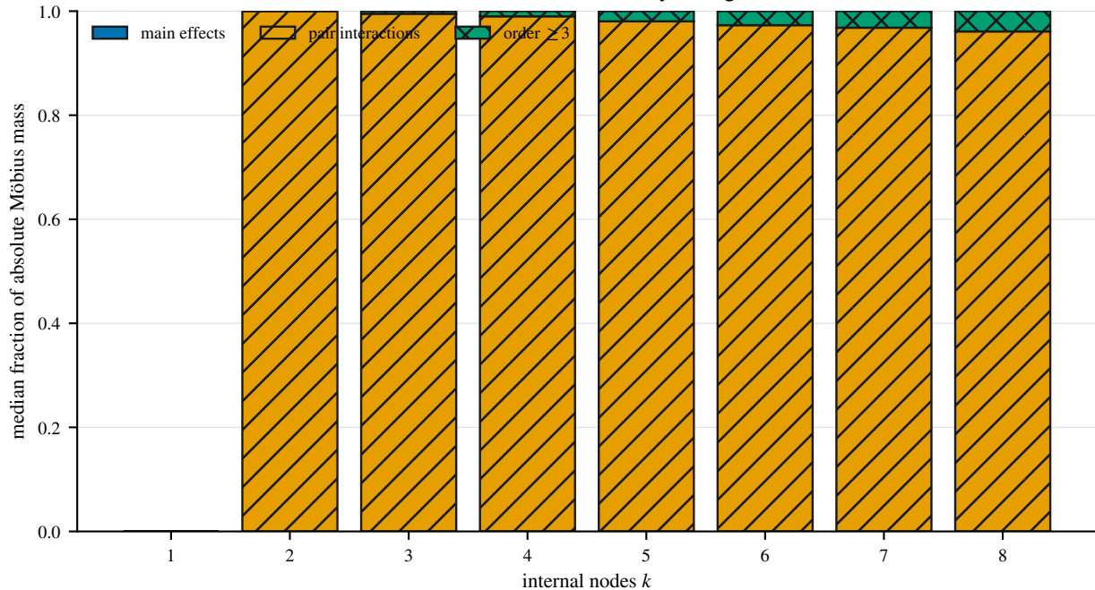
Residual interactions from every leakage mask
