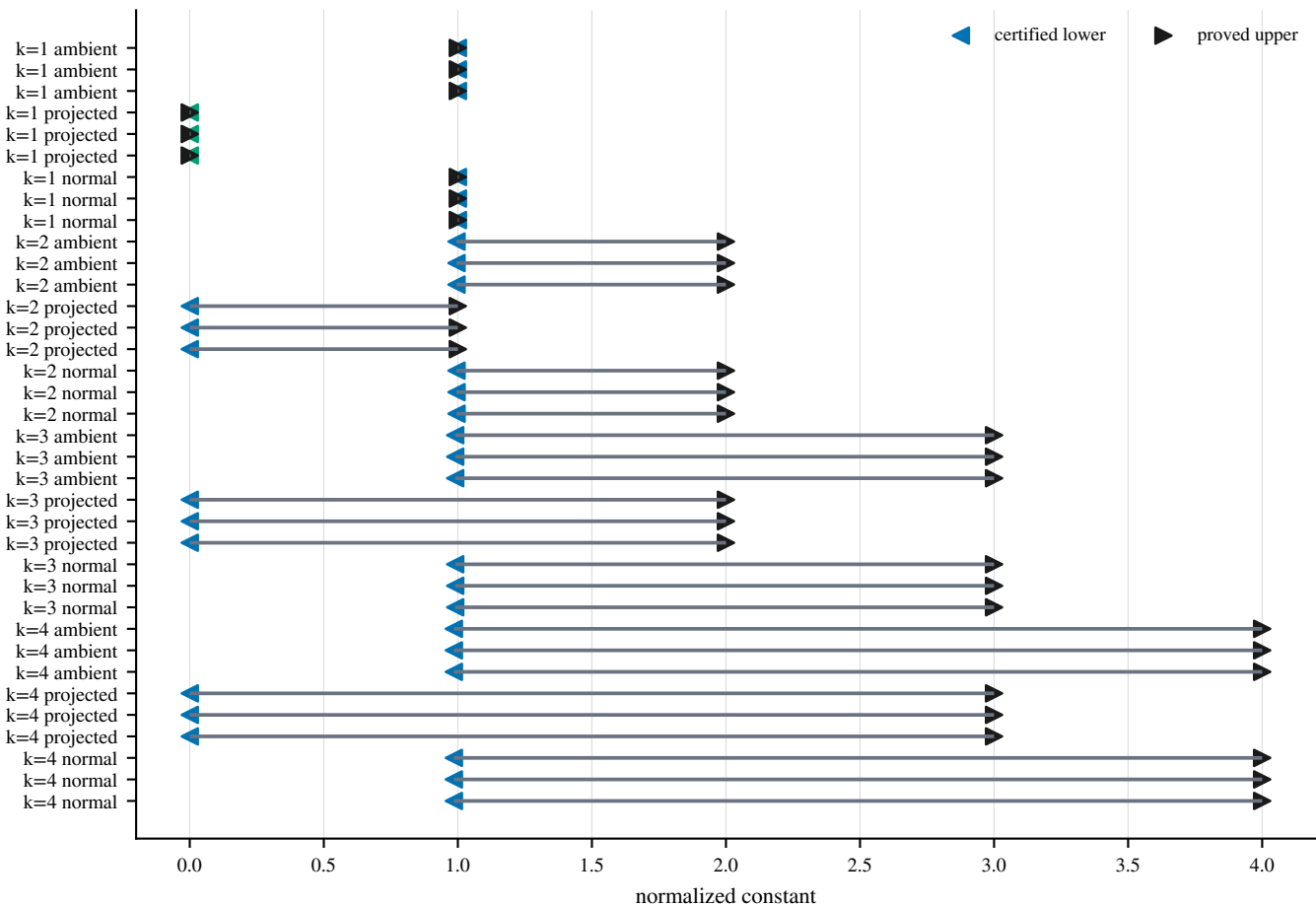
Certified intervals for exact small registered cases
