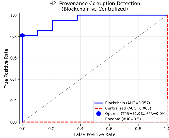
Figure 2: Provenance Verification ROC Curve. Blockchain system achieves AUC=0.957, detecting 81% of tamper attempts. The “Centralized (Mutable)” baseline (AUC=0.0) represents a log immutability test , not detection algorithm comparison: attackers who can modify logs render provenance queries “unverifiable” regardless of detection quality. Results: seed=42, 50 rounds, 30% attack probability.
