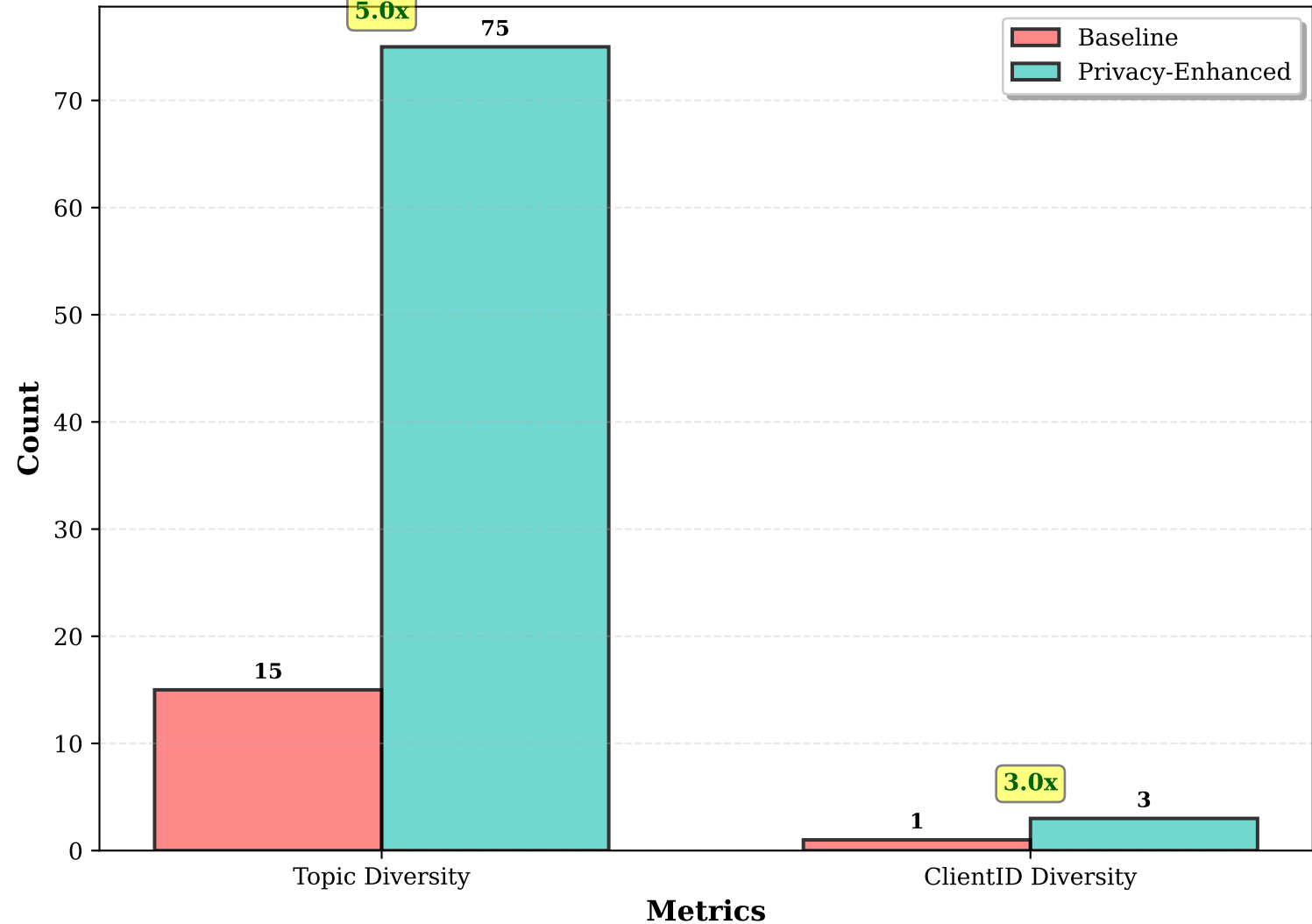
Figure 4.3: Privacy Metrics Comparison
