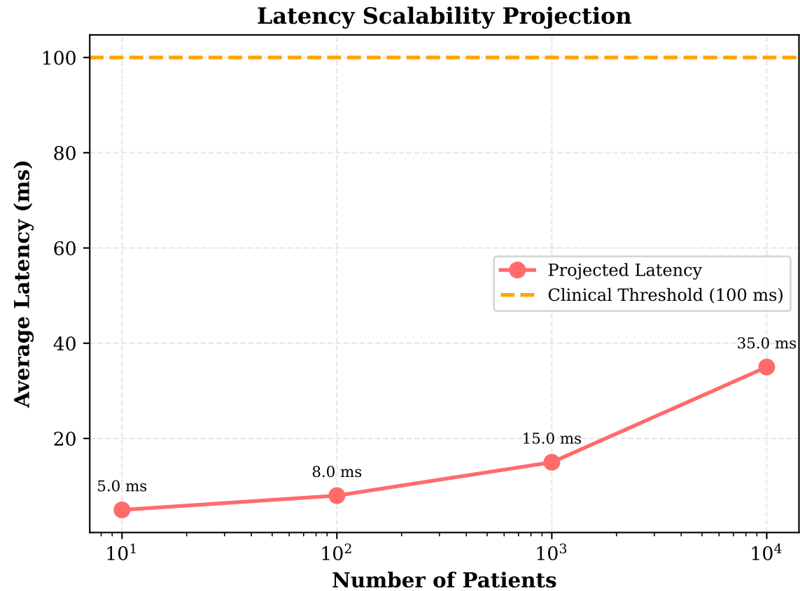
Figure: Scalability Analysis for HPC Deployment
