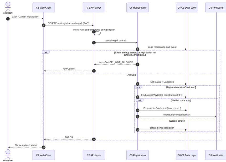
Figure 5: Sequence diagram SD-3 - cancellation with FIFO waitlist promotion
