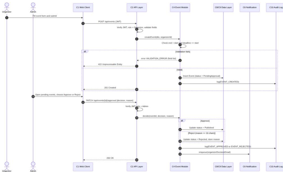
Figure 4: Sequence diagram SD-2 - Organizer creates event, Admin approves
