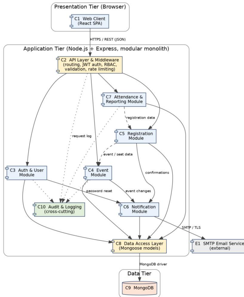
Figure 1: UML component diagram of EMS
