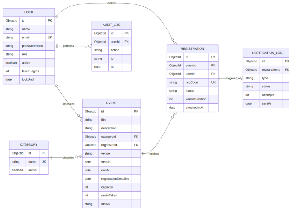
Figure 2: Data model (collections and relationships)
