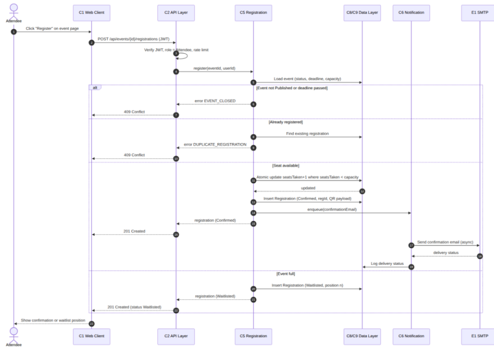
Figure 3: Sequence diagram SD-1 - Attendee registers for an event
