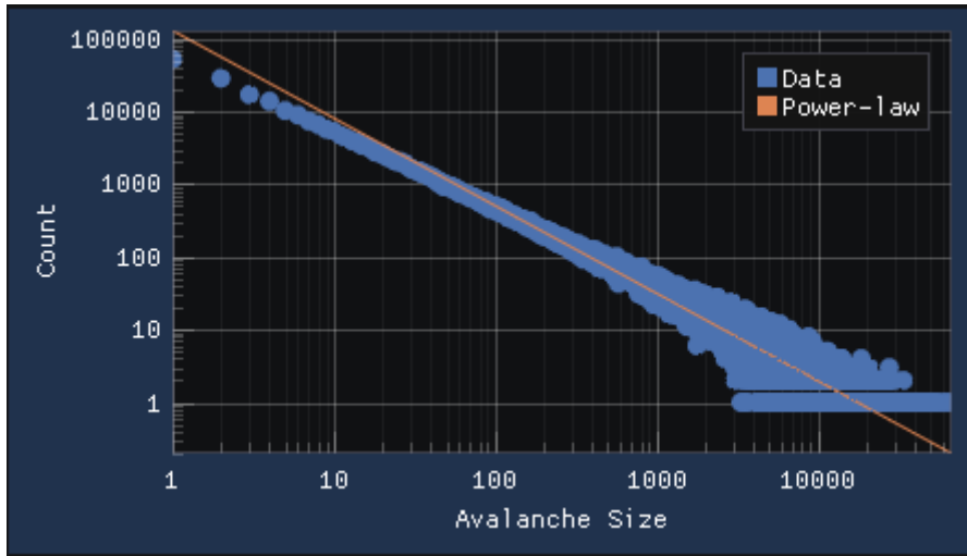
Figure 5: The distribution of avalanche sizes on a square lattice shown on log-log plot.
