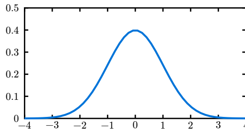
Figure 1: Normal distribution plot.
