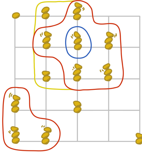
Figure 4: Example clusters on a square lattice. Every cluster is bounded by a red border. The numbers show the size of vertex for respective number of grains. There are two clusters, one of size 3, other of 6. Avalanches are represented as yellow borders extending the red. Avalanche sizes are 3 and 8 respectively. If grain is dropped onto the vertex with blue outline, the avalanche size is 9.
