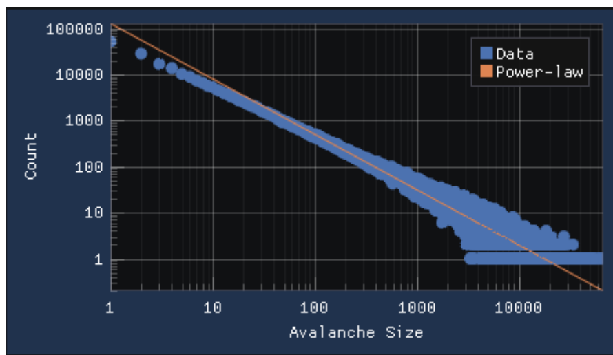
Figure 5: The distribution of avalanche sizes on square lattice G(n) , n = 10.000 on log-log plot with over one million grains dropped.
