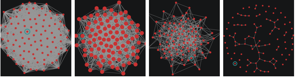
Figure 8: Comparing ER G(n, p) graphs with (from left) p = 0.5 , p = 0.25 , p = 0.1 and p = 0.01 .
