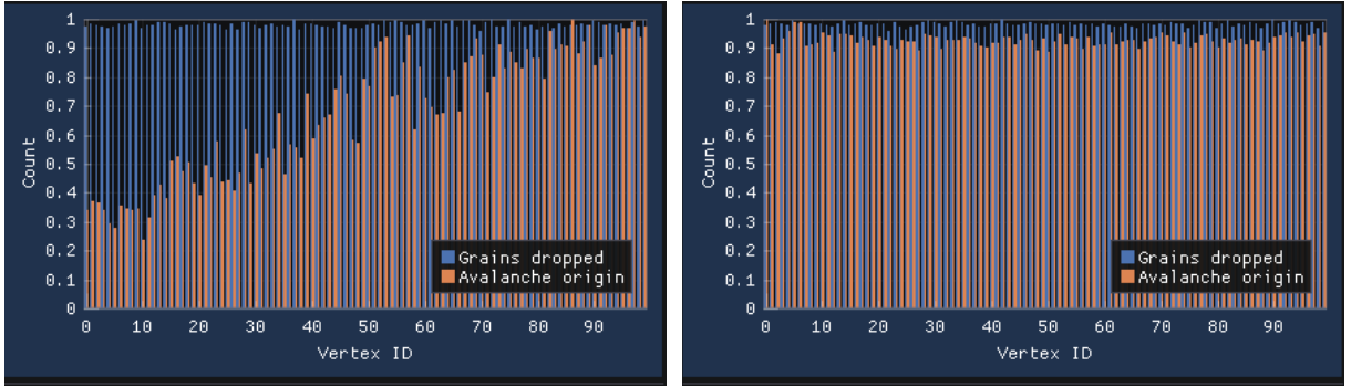
Figure 9: The avalanche distribution graph for BA generated graph with n = 100 , m = 10 . Blue bars show normalized count of grains dropped to vertex. Orange bars show normalized count of avalanches started at that vertex. Vertices with lower ID were added to the graph earlier during generation.
