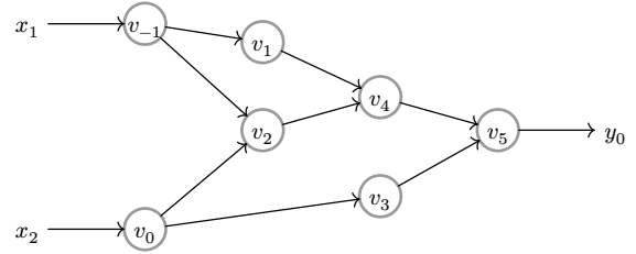
Fig. 1. Computational graph for simple example function.
